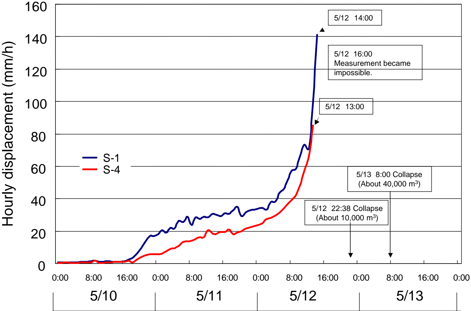
Change of landslide displacement at Higashi-Yokoyama along the Ibi River (measurement: extensometer)
